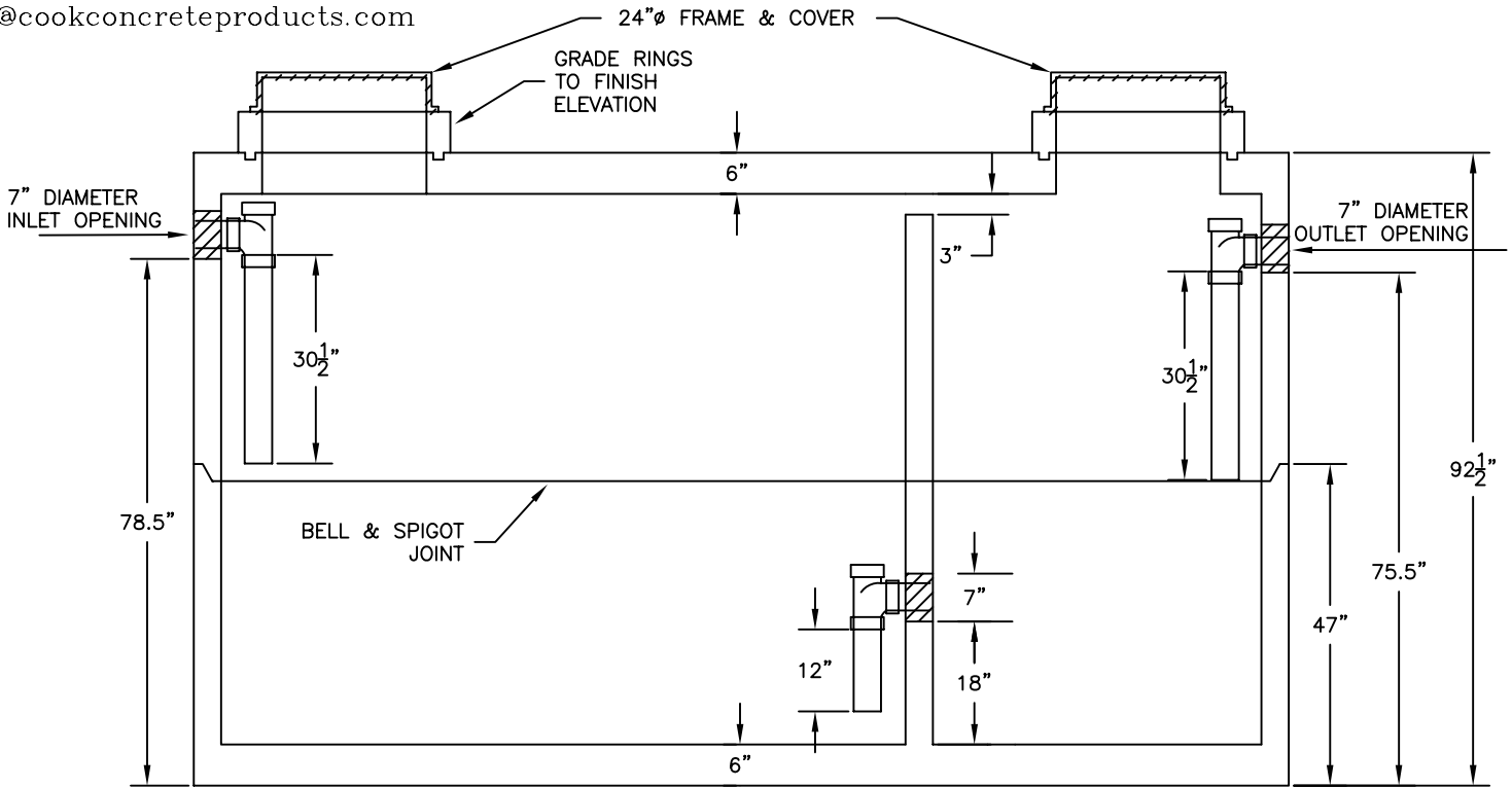
SECTION VIEW
