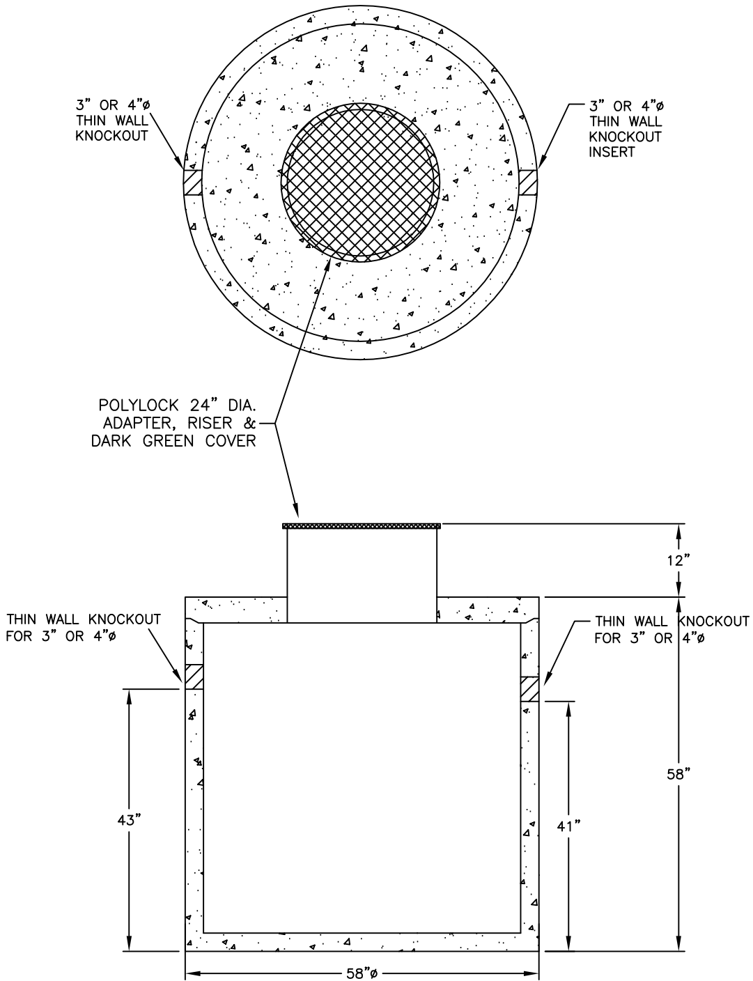
400 GALLON PUMP TANK
