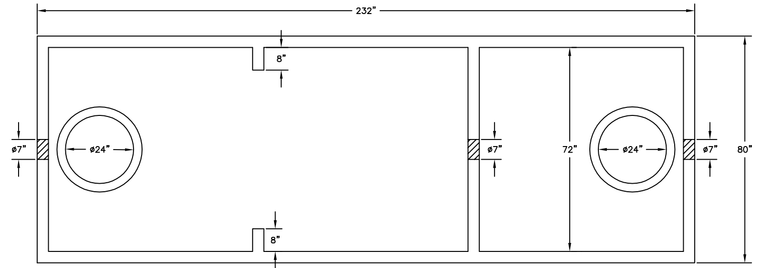
PLAN VIEW
