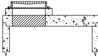
FLAT TOP FOR SHALLOW MANHOLES
