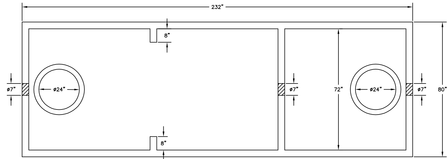
PLAN VIEW
