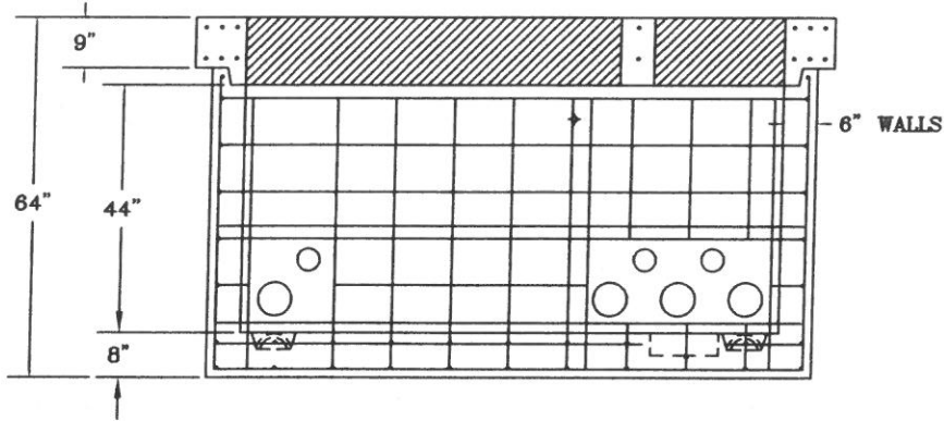
SECTION VIEW
